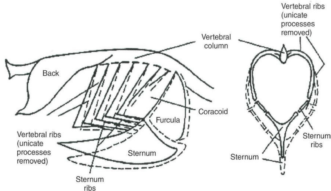
Fig. 14.13. Changes in the thoracic skeleton during respiration in birds. Solid lines show thoracic position at the end of expiration; dotted lines show position at the end of inspiration (Reprinted from Whittow, 2000. Used by permission of the publisher.)
